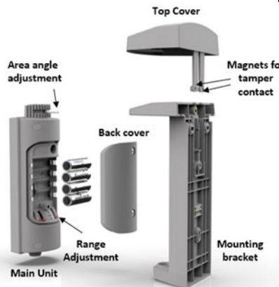
FIG. 1 - DETECTOR PARTS
