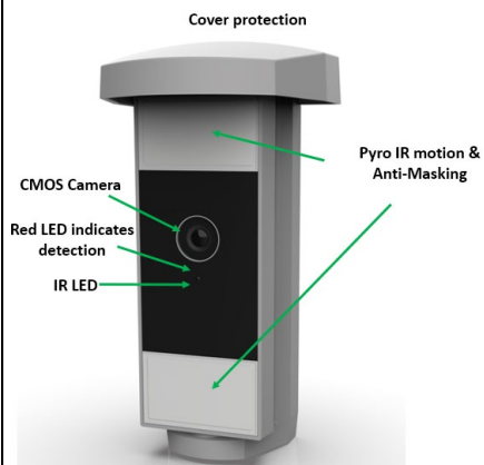
FIG. 2 - PRODUCT OVERVIEW
