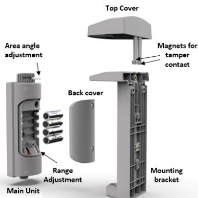
FIG. 1- DETECTOR PARTS
