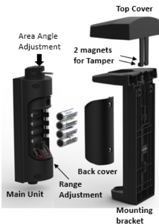
FIG. 2 - PRODUCT OVERVIEW
