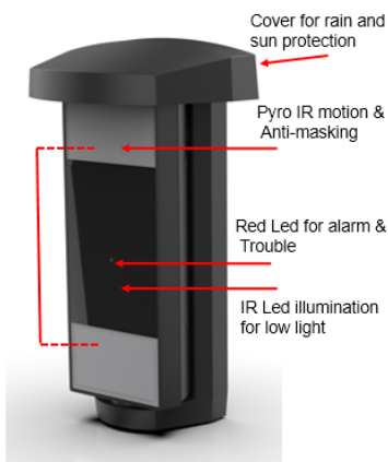
FIG. 2 - PRODUCT OVERVIEW
